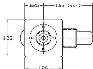
Illustrated is the M-61 Model with 3/8" flare fitting.
