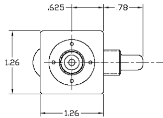
Illustrated is the M-61 Model with 1/4" flare fitting.
